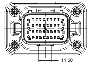
Receptacle - Key C (ATV04-38PC-Sx)
